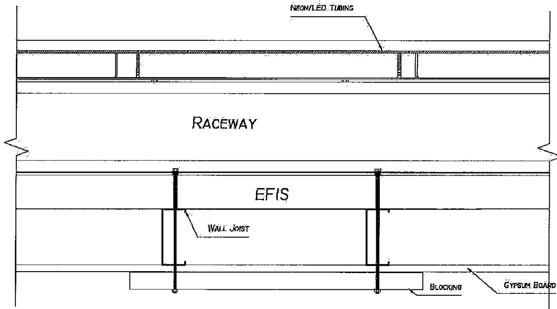
PLAN VIEW SCALE 1 1/2" - 1'-0"
