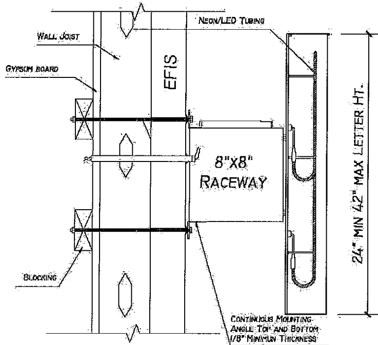
SECTION CUT SCALE 1 1/2" - 1'-0"
